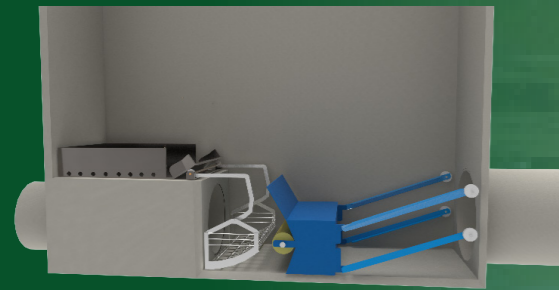
In addition to a floating capture system (Orléans - Loire)
